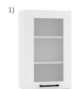
WS40 P/L /72 400x720x300 WS45 P/L /72 450x720x300 WS50 P/L /72 500x720x300 WS60 P/L /72 600x720x300
